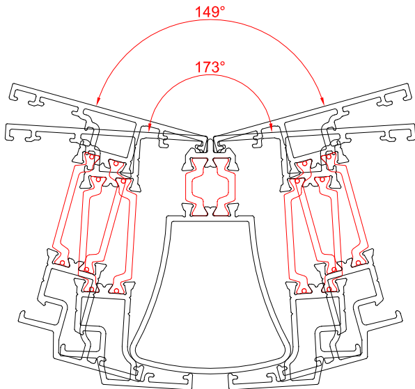
T0184 Bay Post Small ( 2 )
