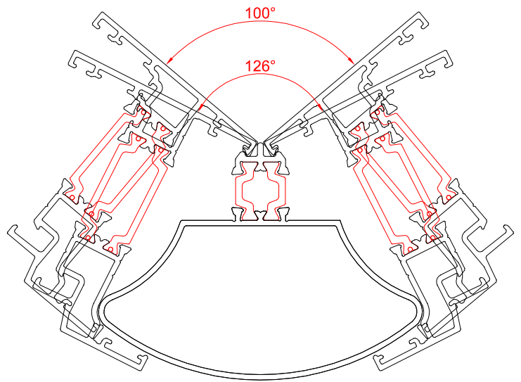
T0186 Large Bay Post
