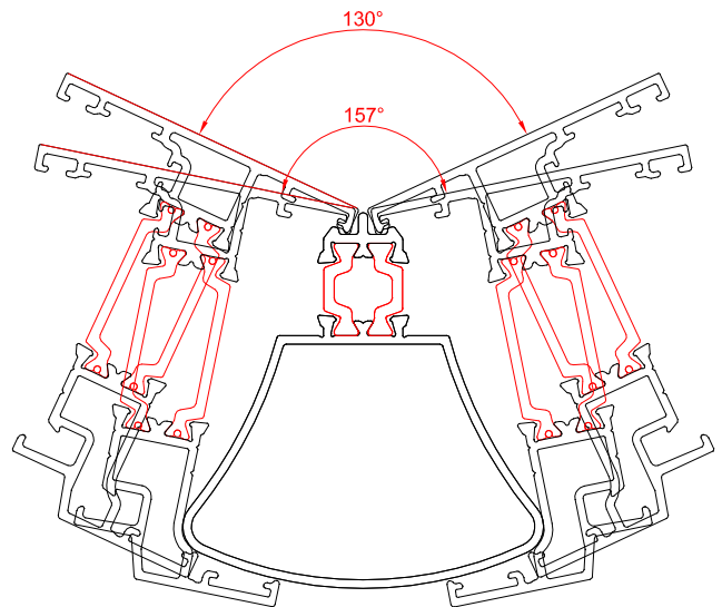
T0185 Bay post Small ( 1 )
