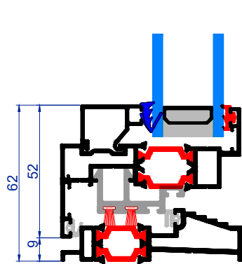
Bottom Rebated Lowthreshold
