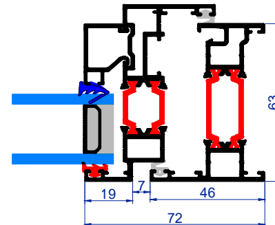
Single Door Lock Stile
