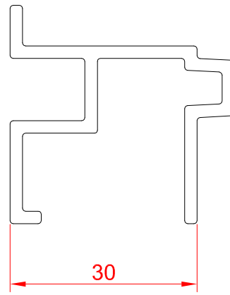
Cill extension 107131
