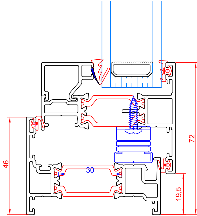
C202 Slim Outer - C206 Vent - C211 Bead
