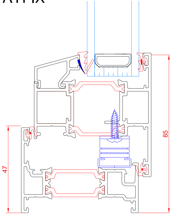
C202 Slim Outer - C205 Vent - C212 Bead
